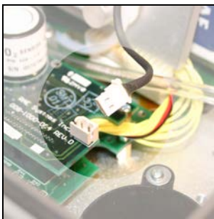
Figure 7-7 Gas plate connector
